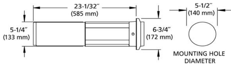
Mounting specifications for SF2000 Cup Dispenser
